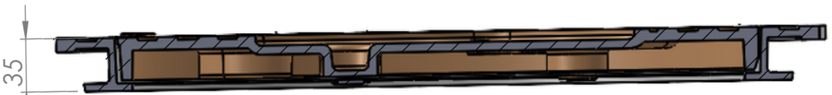
SECTION C-C SCALE 1 : 3.5
